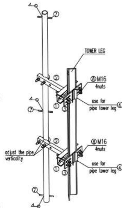
BACK VIEW
