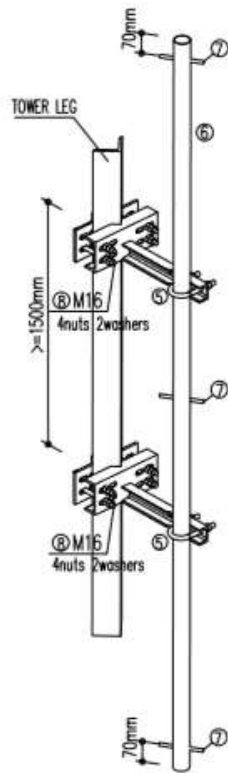
FRONT VIEW
